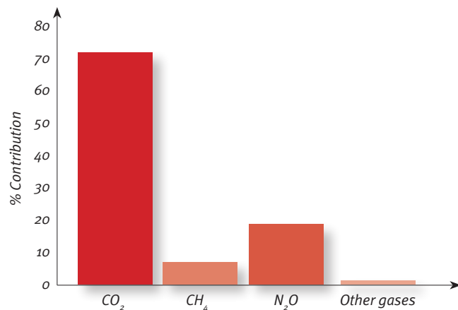
Relative contributions of different green house gases to global warming
