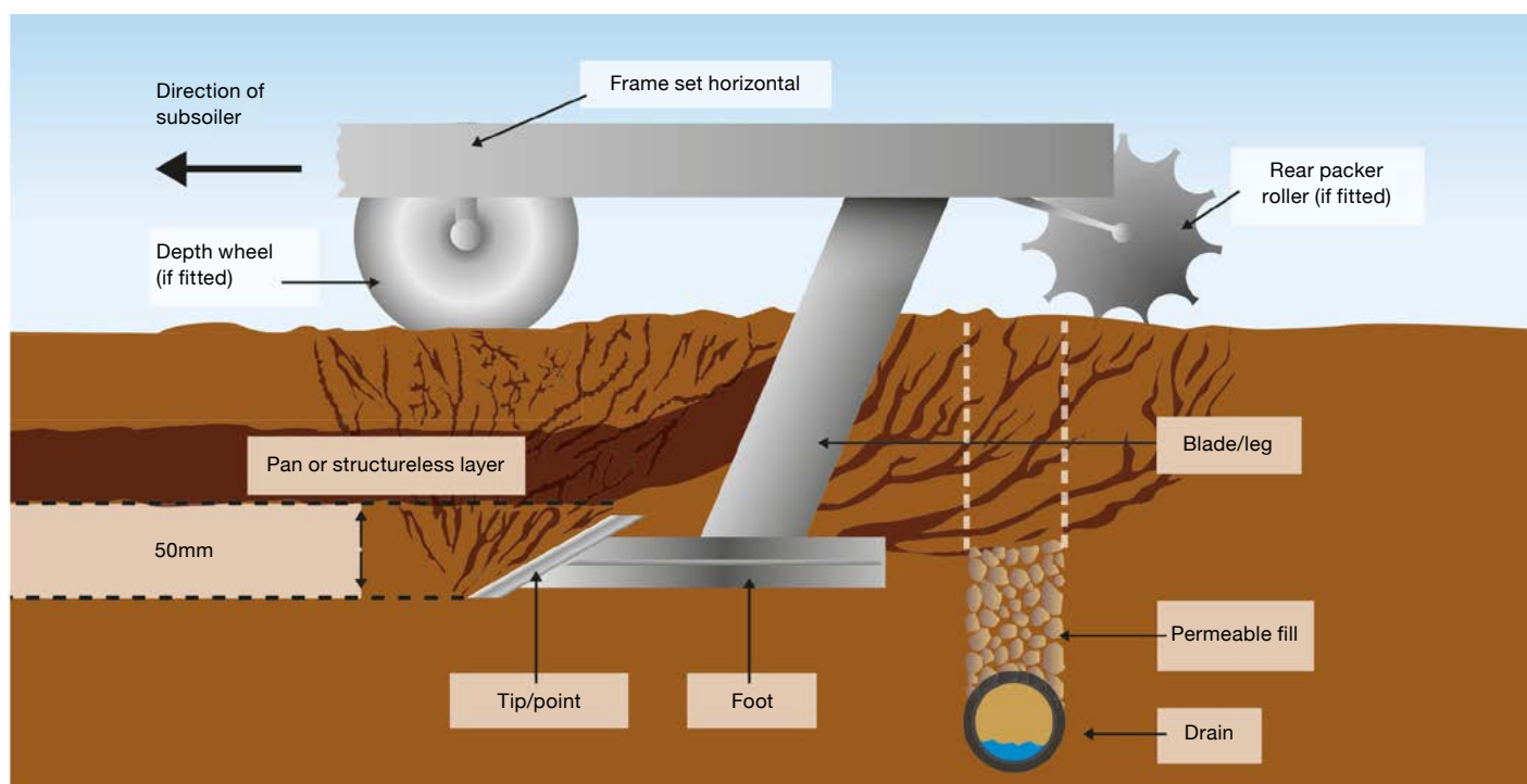
Figure 13. Subsoiler operation
