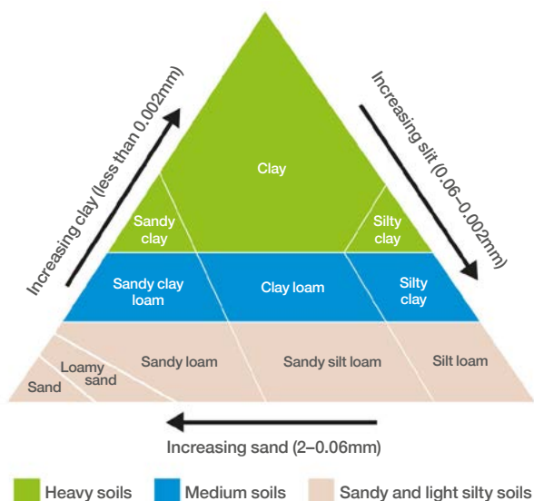
Figure 25. Soil texture classification
