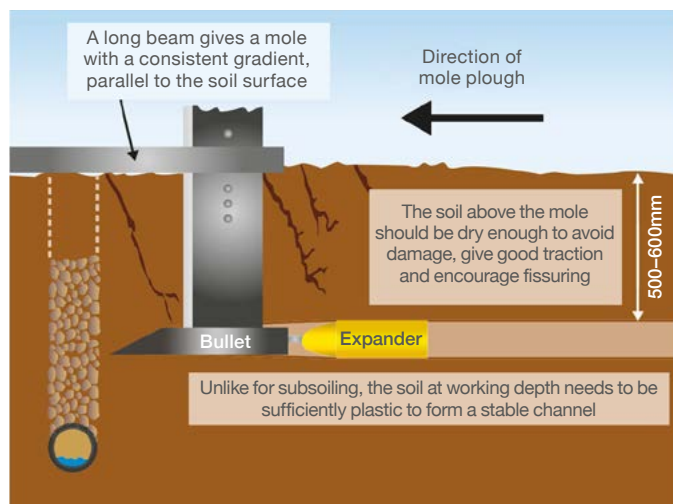
Figure 26. Appropriate conditions for forming mole drains
